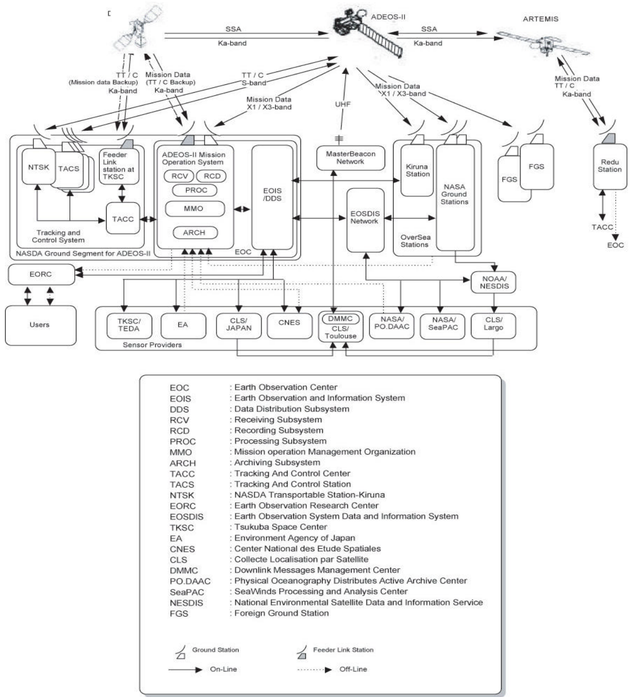
Figure 4-1: ADEOS II Data Flow
